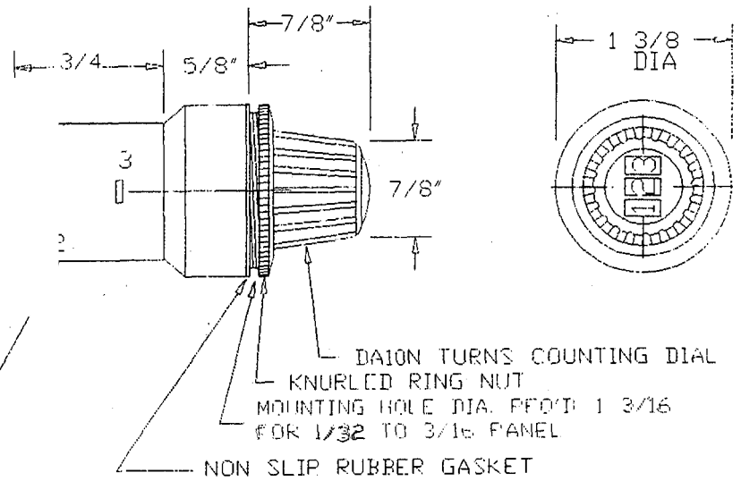
MW22 POTENTIOMETER
